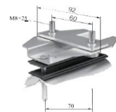
C Track Hanger
