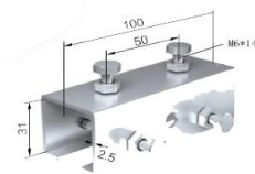
C Track Joint
