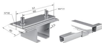
C Track Hanger
